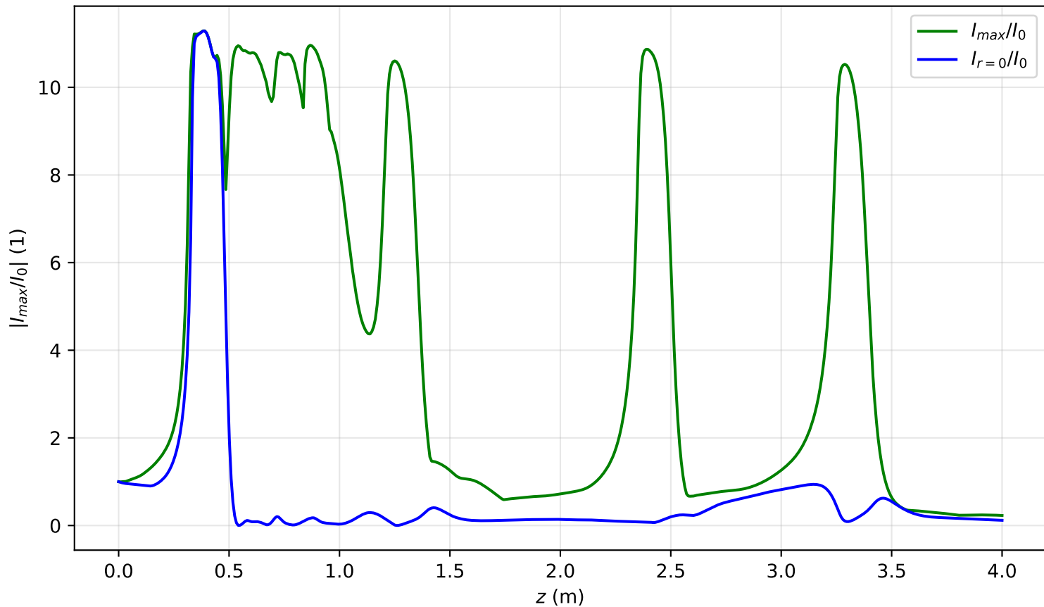
I_{max}(x=0, y=0, z)/I_0 , \text{Pin}=9.9\text{Pcr} , noisy input, artificial time
